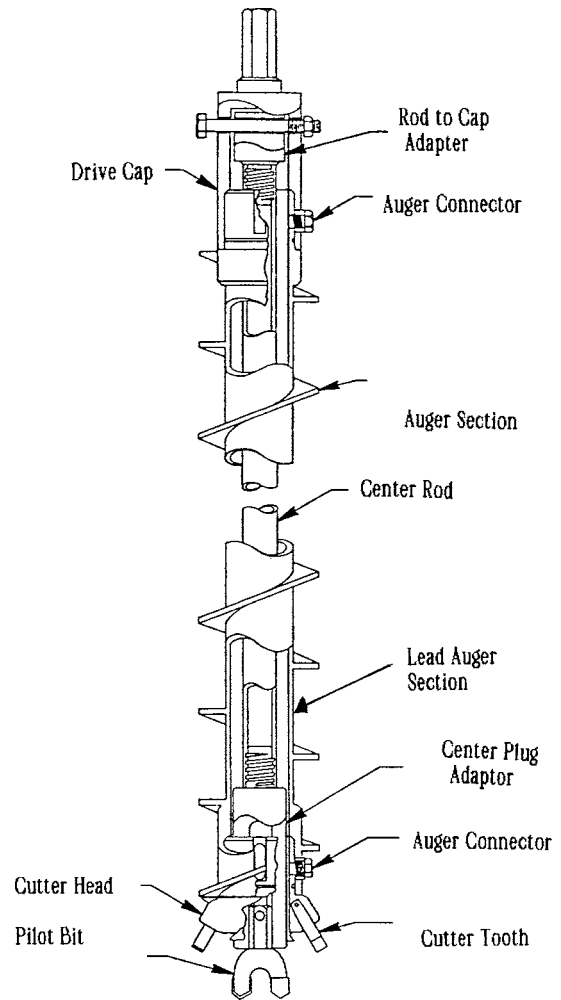
FIG. 1 Rod-Type Auger System With Pilot Bit 1
